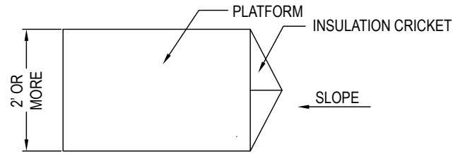
CRICKET PLAN VIEW
