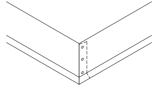
CLOSED CORNER FLASHING SET IN BED OF URETHANE & FASTENED W/SPECIFIED FASTENERS
